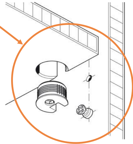
System Bolt Single H.262.20.985 'Single bolt for Fixed Shelves. Cam system Locks onto this Bolt. Place on end Gables/Panels
