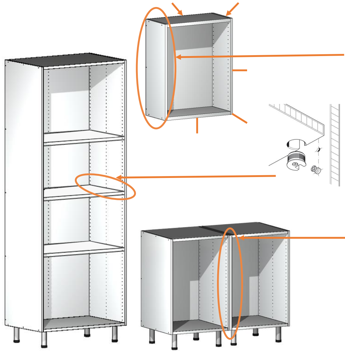
Flush Rail Cam H 263 02 105 "Cam System for Fixed Shelves. 4 Cams per Fixed Shelf. Screws onto single or double bolt system. System Bolt Single H 263 02 965 "Single bolt for Fixed Shelves. Cam System Locks onto the Bolt. Place on end Gables/Panels.
