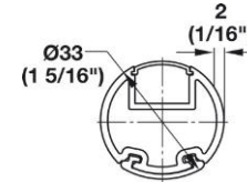
LED Strip Lighting Closet Rod WW
