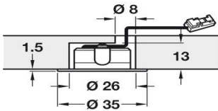
1 3/8" LED Light WW
