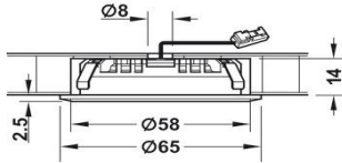
2.5" LED Light WW
